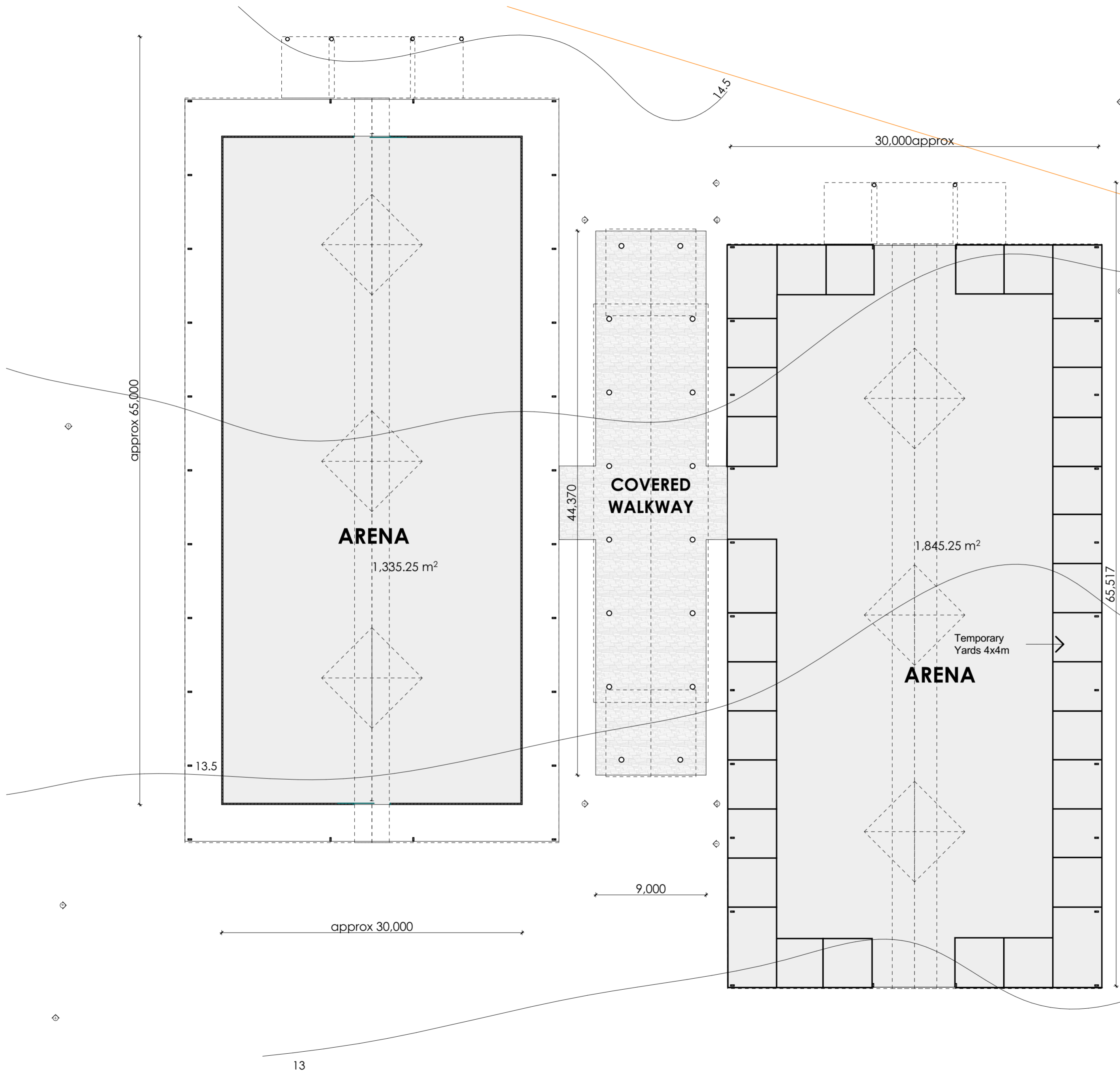
1 Floor Plan Arenas and Walkway 1:250
