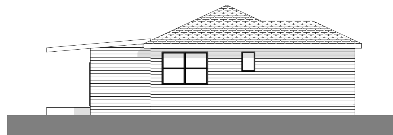
4 West 1:100
