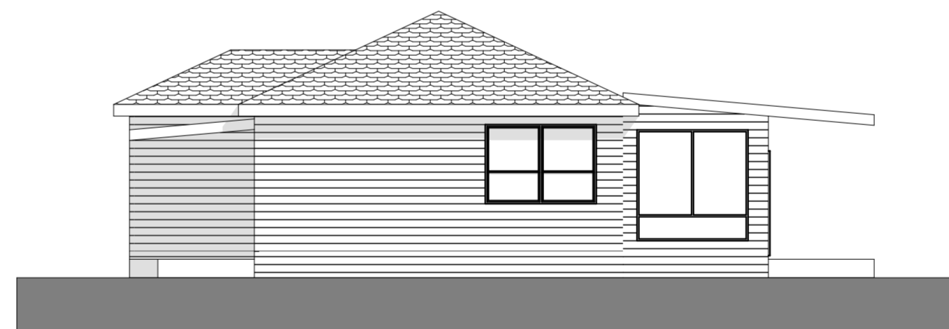
2 East 1:100
