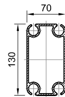
PHC-006 GABLE UPRIGHTS RIDGE & EAVES PURLINS
